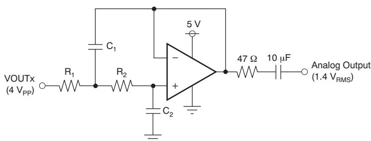
Figure 44. Capless Post-LPF and Buffer Using 5-V Single Supply ( 1.4 \text{ V}_{\text{RMS}} Output) for Noninverting Output
