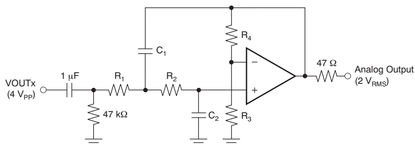
Figure 43. Typical Post-LPF and Buffer ( 2 \text{ V}_{\text{RMS}} Output) for Noninverting Output
